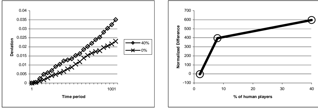
c) 40 % (8 players of 20 agents) d) The scaling of the normalized difference as a function of the percentage of human participants. Figure 1: Cumulative market deviations in runs with and without human players. (The deviation axis shows the values in millions.)
